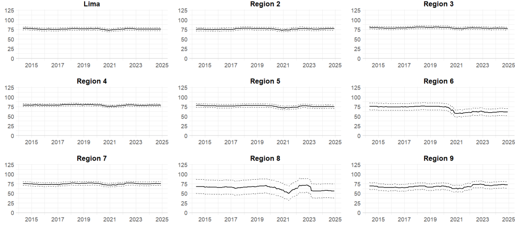
Figure 4: Dynamic spillovers FROM all others in the time domain
