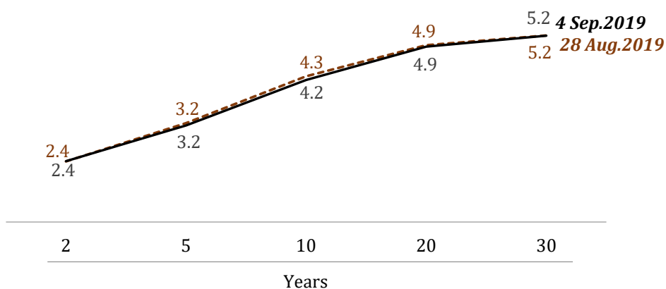
Yield curve of BTP (%)
